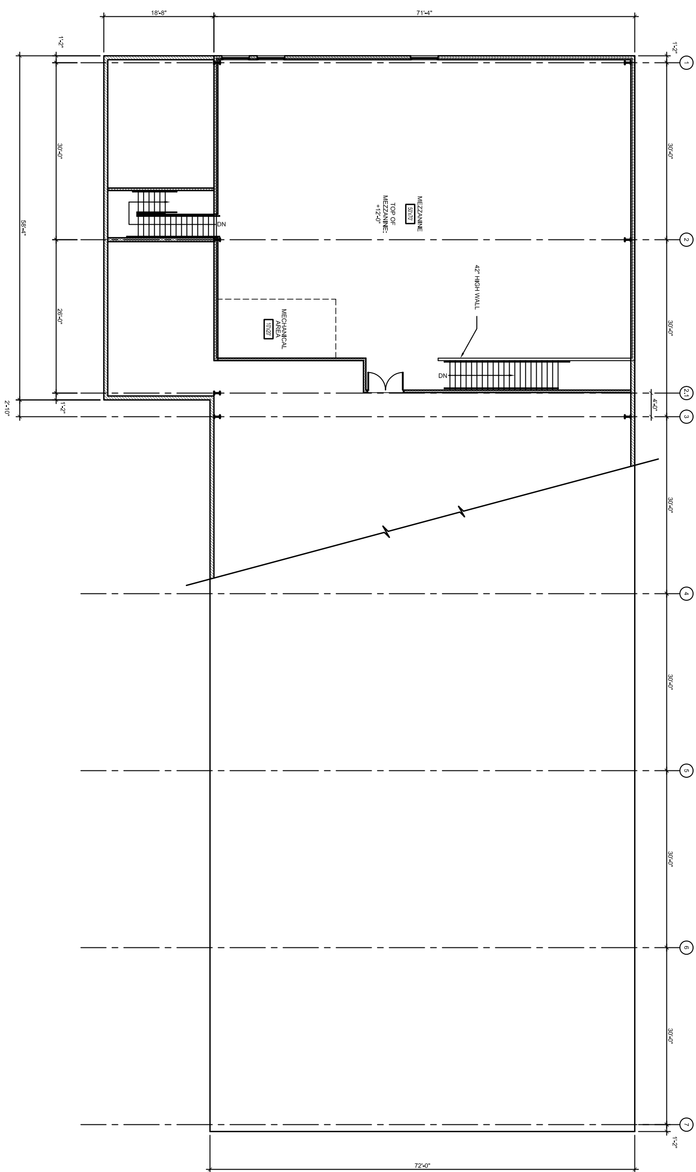
1 MEZZANINE LEVEL FLOOR PLAN A112 1/8" = 1'-0" AREA: 3,986 S.F.
