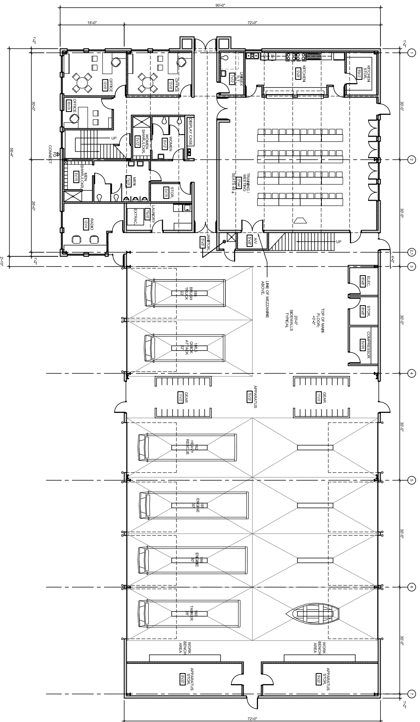
Main Level Floor Plan 14,180 SF ±
